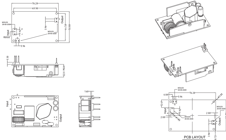
GTM43007-A class I OUTLINE DRAWING FOR 15V,18V,24V,48V
