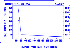
STATIC CHARACTERISTICS
