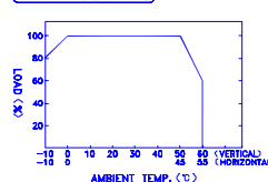
OUTPUT DERATING
